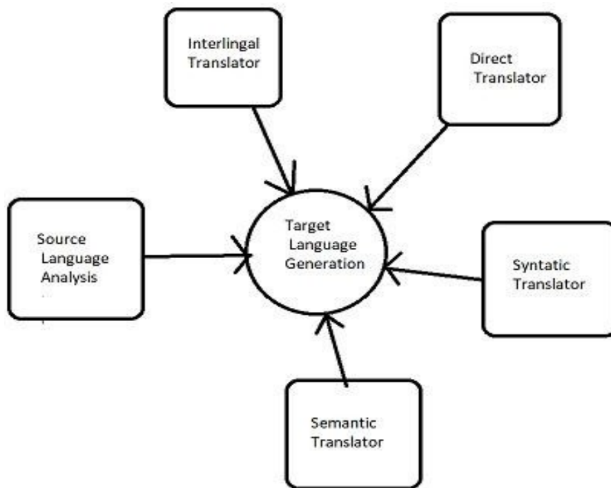
Figure 5.3.1: Level 0 DFD
