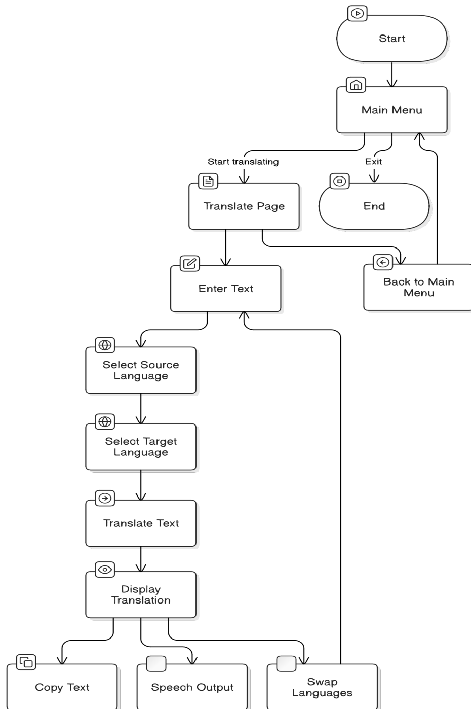
Figure 6.2: Activity diagram
