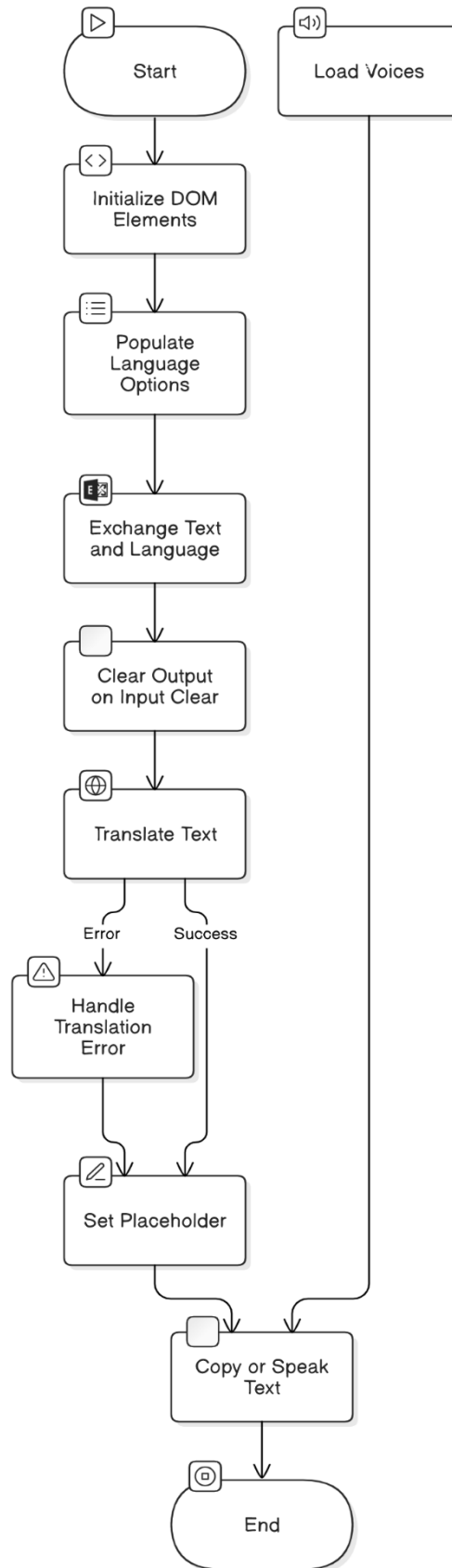
Figure 5.3.2: Level 1 DFD
