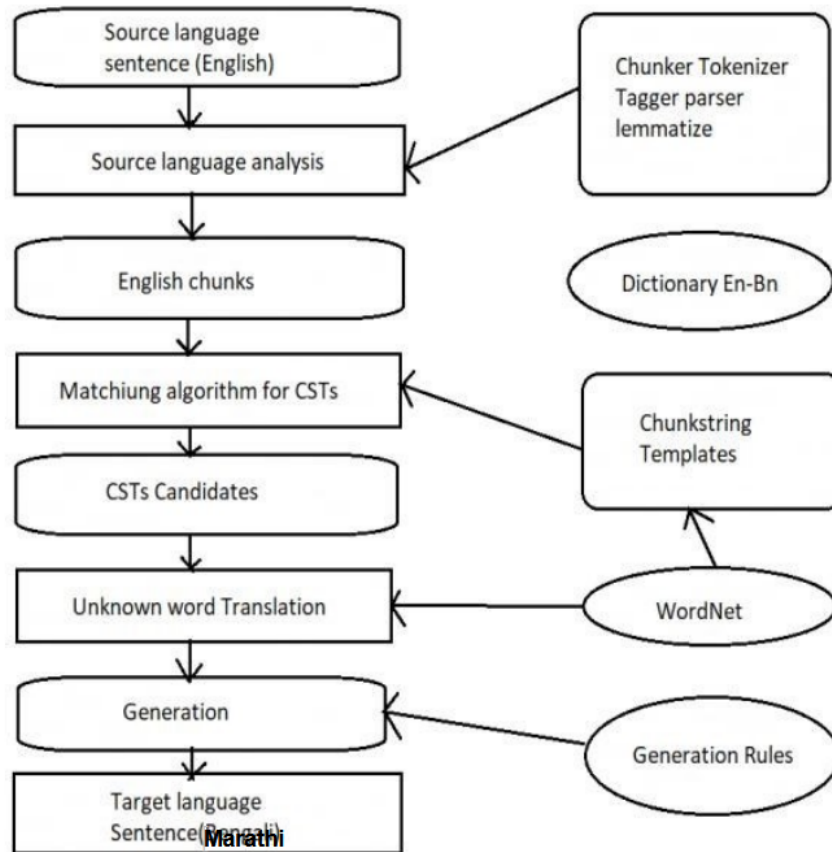
Figure 5.3.3: Level 2 DFD
