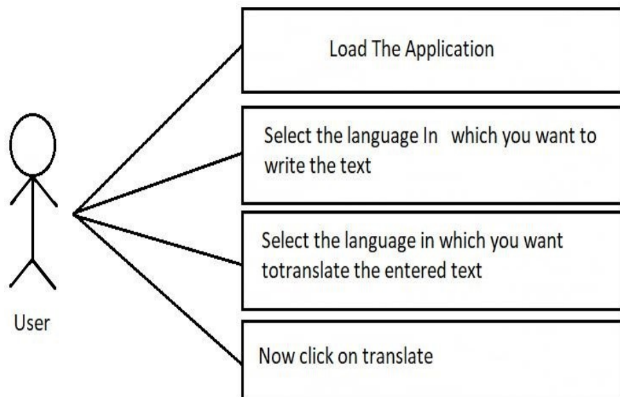
Figure 5.1: Use-case diagram
