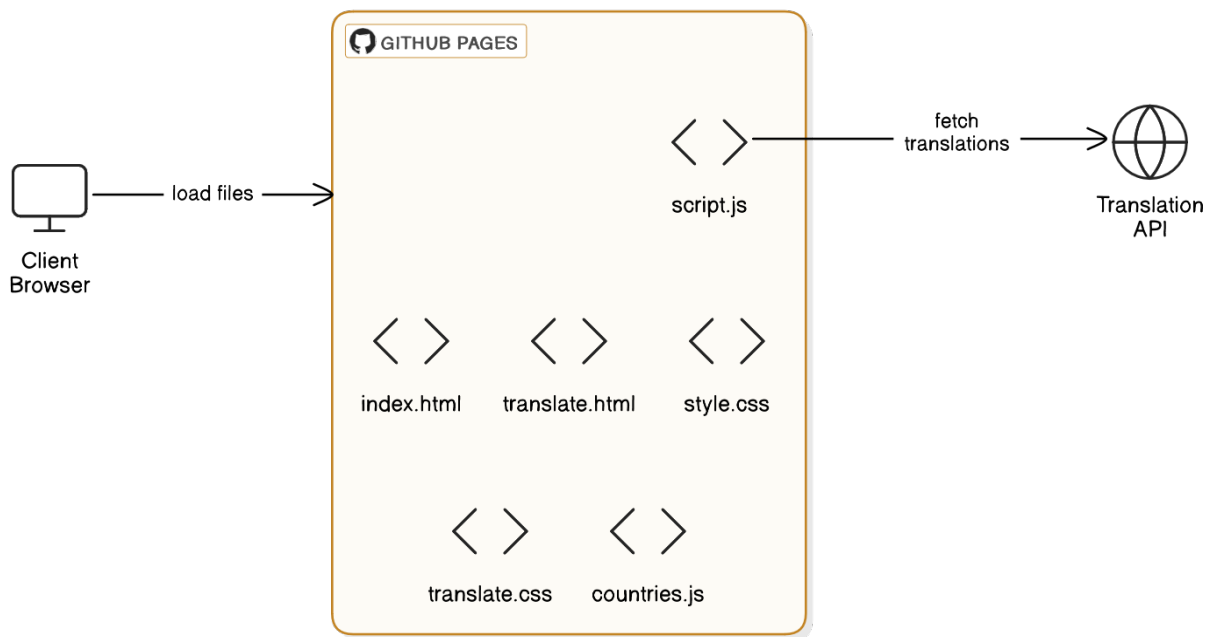
Figure 6.4: Deployment diagram
